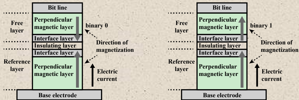
(a) STT-RAM
